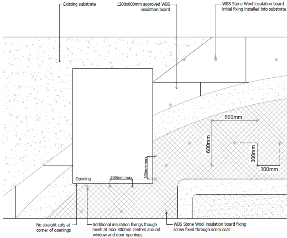
Diagram 1 - Typical mechanical fixing arrangement
