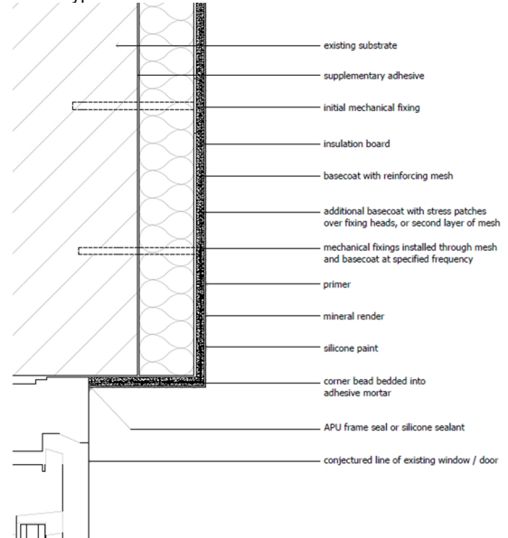
Diagram 9 - Typical window/door head detail
