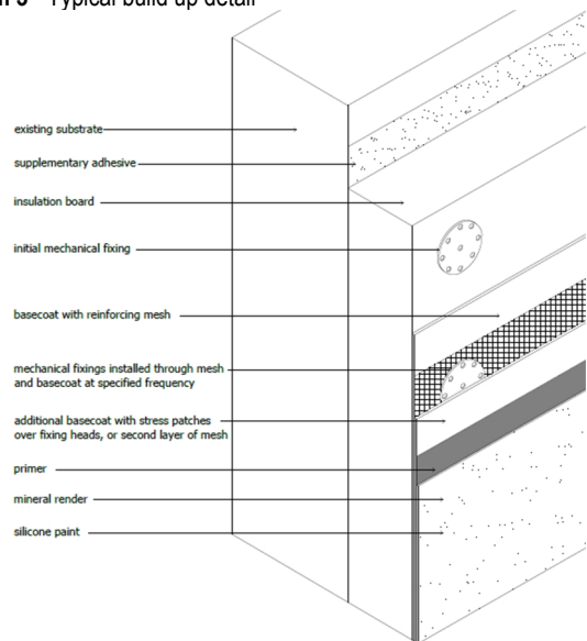
Diagram 3 - Typical build up detail
