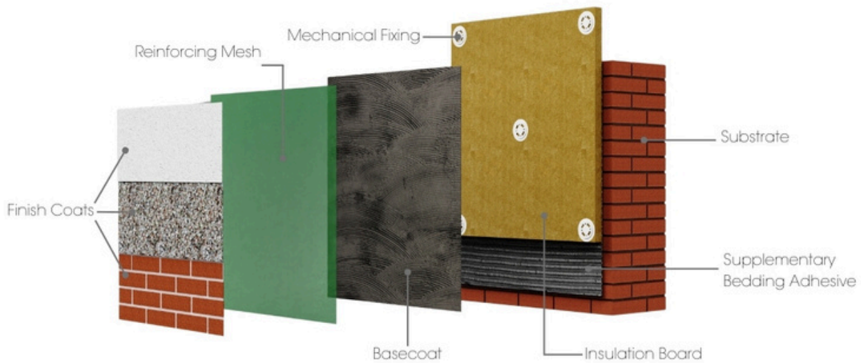
System Build Up 30 Year Durability
